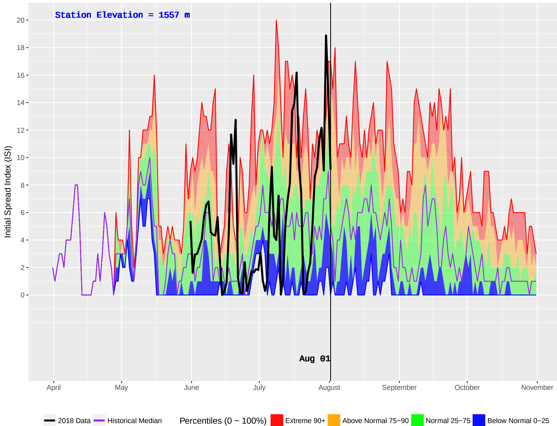
SKOONKA (1024) : Historical (2008–2016) and Current (2018) Daily Initial Spread Index (ISI)
