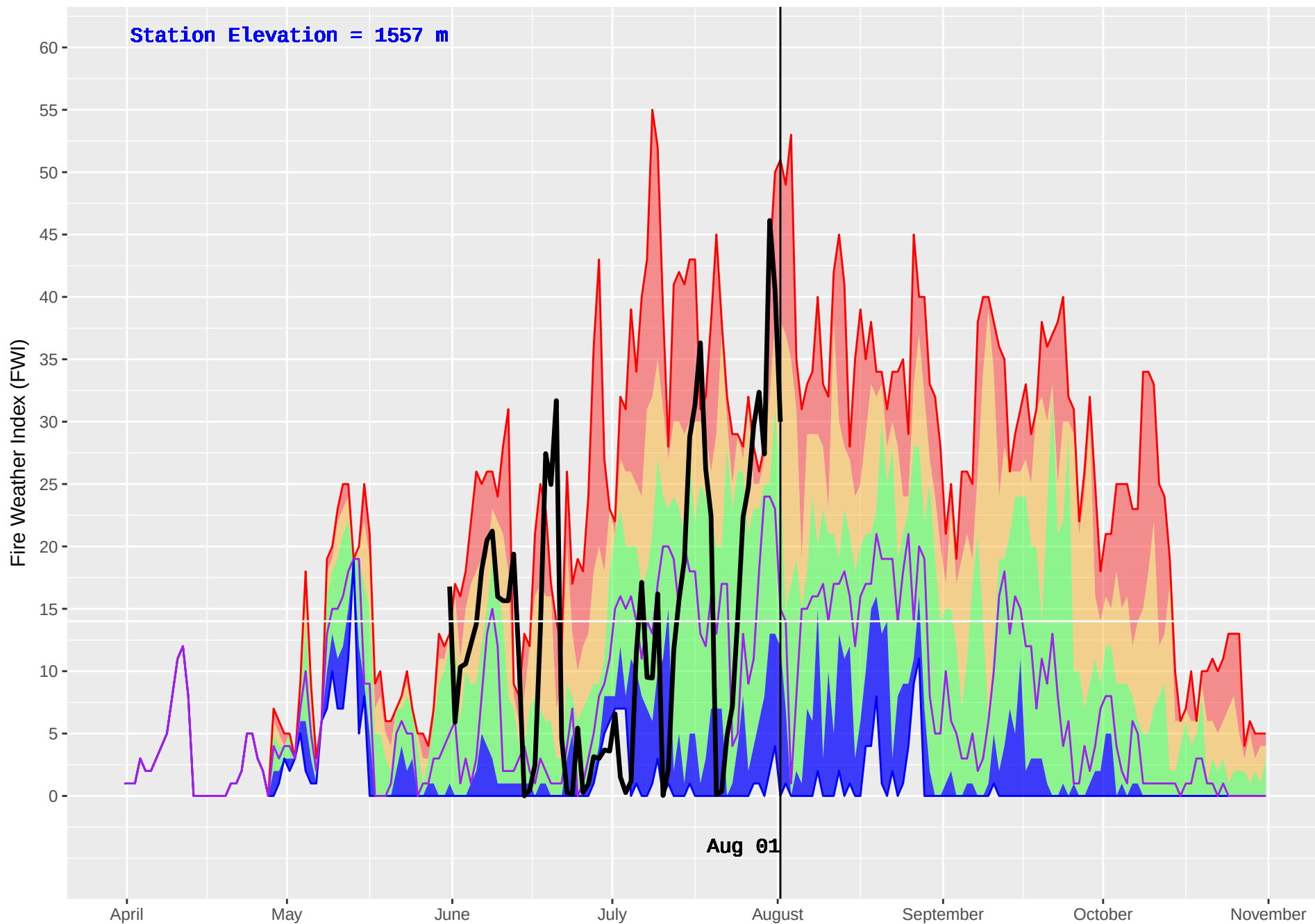
SKOONKA (1024) : Historical (2008–2016) and Current (2018) Daily Fire Weather Index (FWI)
